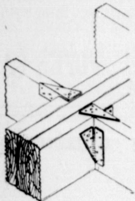
HOW NEW framing anchor grips work to eliminate toenailing in joints.
