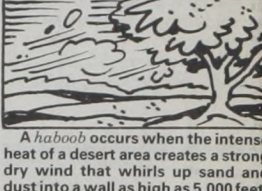
A haboob occurs when the intense heat of a desert area creates a strong dry wind that whirls up sand and dust into a wall as high as 5,000 feet.
