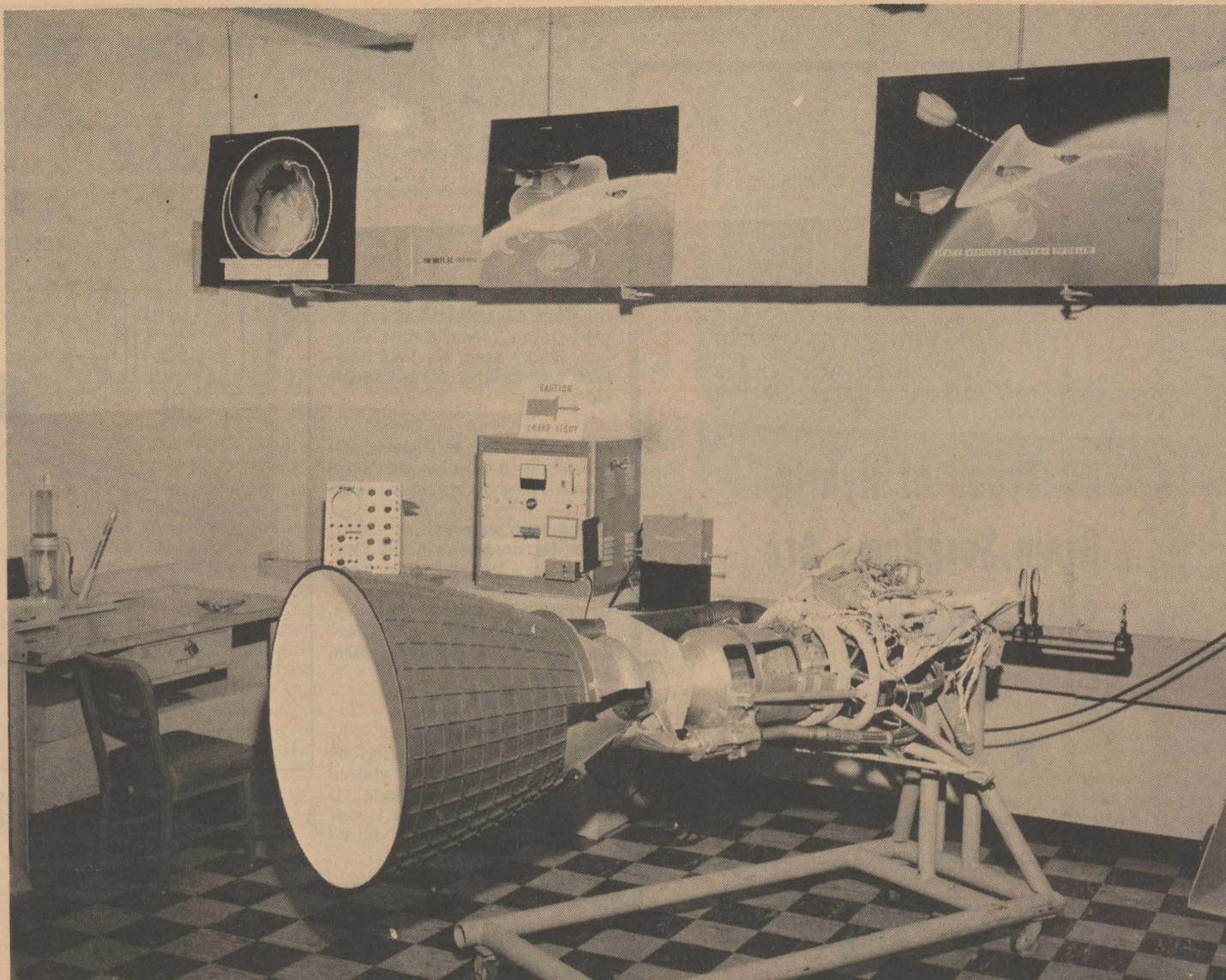
AGENA ENGINE CUTAWAY--This Agena liquid rocket engine cutaway with re-entry technology systems in the background as well as many other rocket and missile components will be on display at Reese Air Force Base, Armed Forces Day,
