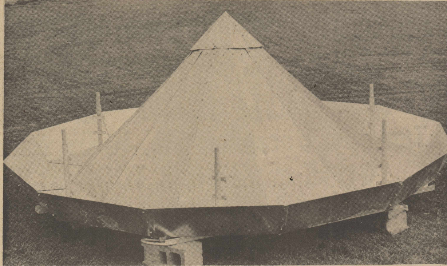
WHAT'S IT????---Nope. It's not a flying saucer, and it's not a ladies' hat. It had people guessing for awhile as they passed by, but upon completion it turned out to be a stock feeder being constructed by Olton Farm Supply.
