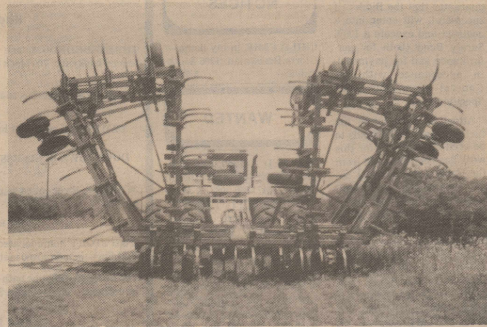
THIS FRIGGSTAD Chisel Plow is 80 ft. wide and each shank has its own spring. Farm Operations manager Charles Durham of Knox City explained that one Big Bud will do the work of three tractors, using only half as much diesel.
