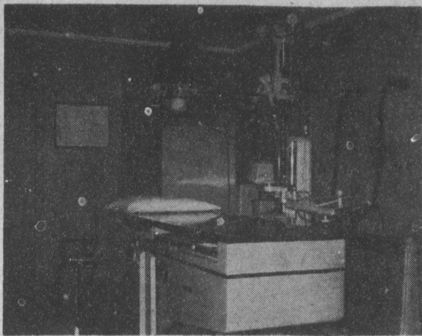
The X-ray Machine is a 500 milliamper Westinghouse with tilting table and separate fluoroscope tube. According to the manufacturer there is only one other machine of this type in South Texas, located at Memorial Hospital in Corpus Christi, Texas.
