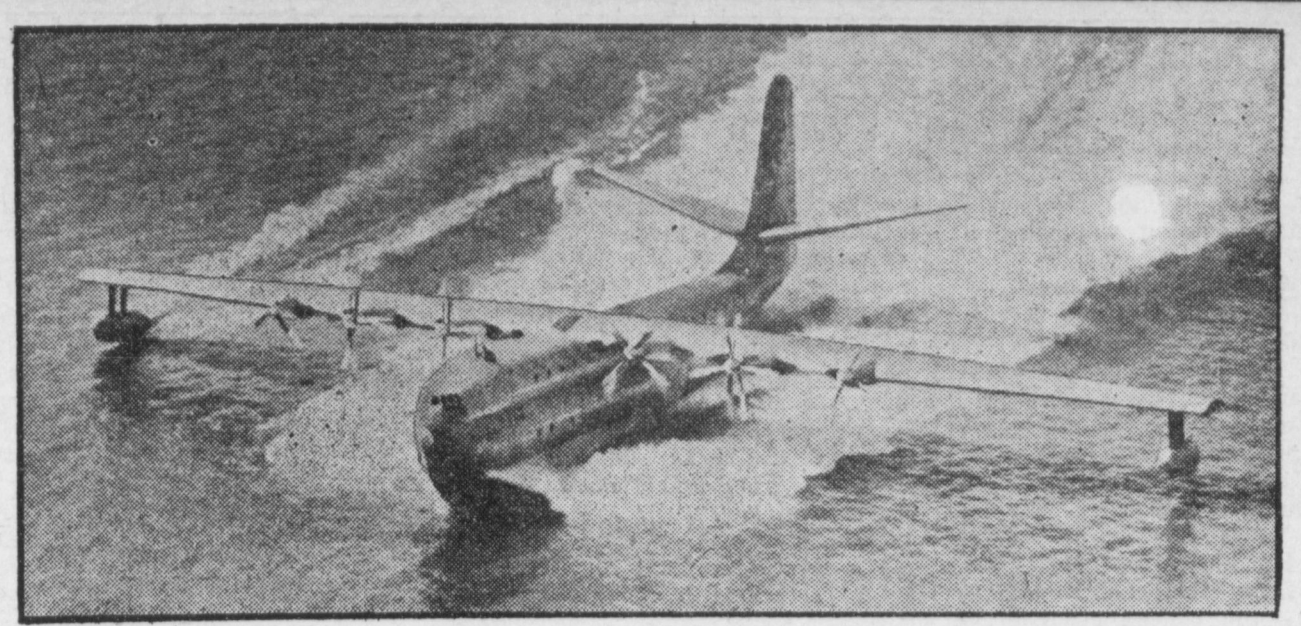
TAKING TAXI-TESTS - Britain's giant flying boat, Princess, is seen above in the midst of taking test runs off the Isle of Wight. Thunder of the 10 Proteus prop-jet engines was reported heard several miles away as the big ship circled the island in test flights. Weighing 140 tons, she has a wing span of 219 feet, is 148 feet long.
