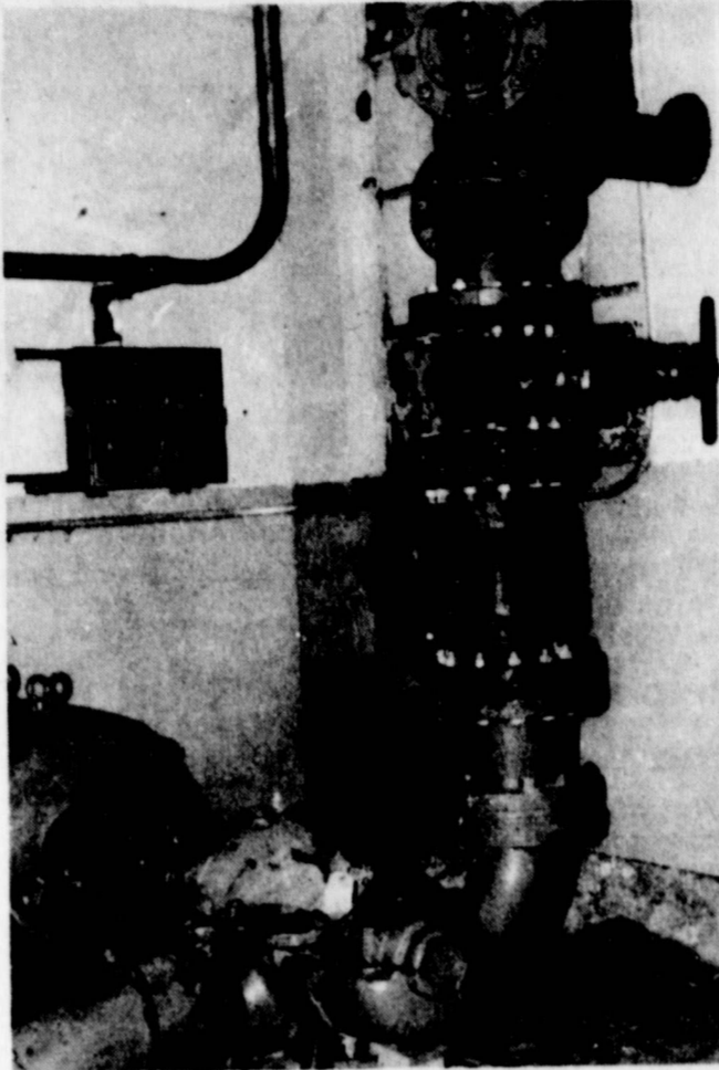
ONE OF TWO old water pumps inside the pump station at the lake is shown above. City Manager Mike Moore stated that during high water usage times such as summer months, one of the pumps is required to run 24 hours a day, just to keep up with the water usage. Both of the pumps will be replaced under the new system, providing adequate water pressure to the city at all times. (staff photo)
