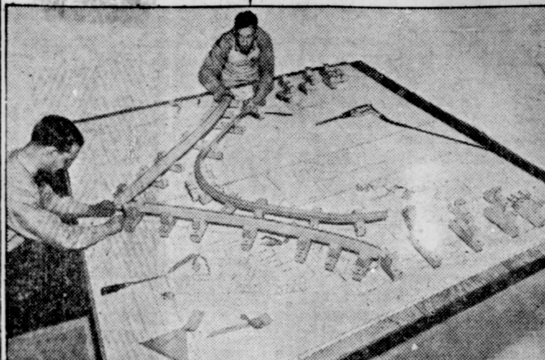
TO SPEED DEFENSE ... Aircraft engineering's newest ally in national defense speed-up is process shown being used in Glenn L. Martin plant by which drawings for parts are photographed, full size, and printed directly on large sheets of aluminum alloys with sensitized surface. Parts can be cut directly from material itself, or full-size parts built, as above, just by following lines on giant photo-print.
