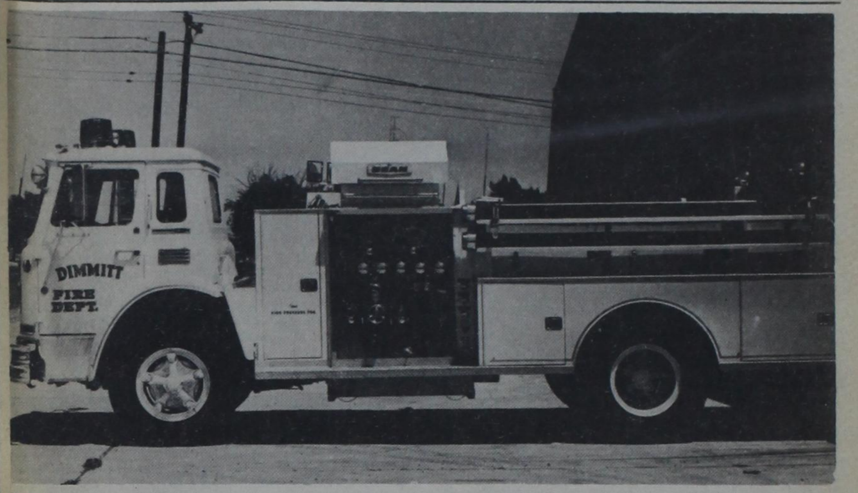
NEW PUMPER — Dimmitt's new 500 gallon pumper unit arrived in the city Friday. City Fire Marshall Guy Waldrop and fireman Rex Cowart shuttled the truck to Dimmitt from the John Bean plant in Tipton, Ind. The white unit features high pressure and volume pumps which can both be operated at the same time if necessary. The cab-over design of the truck allowed extra storage compartments to be installed to the rear of the cab.
