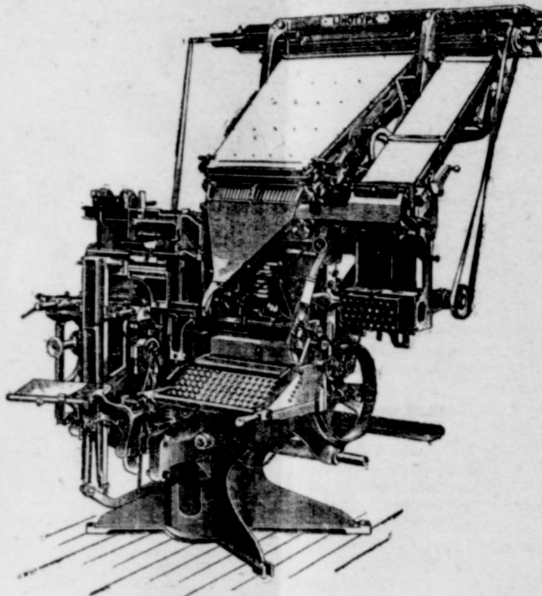
THE MODEL 19 MERGENTHALER LINOTYPE
