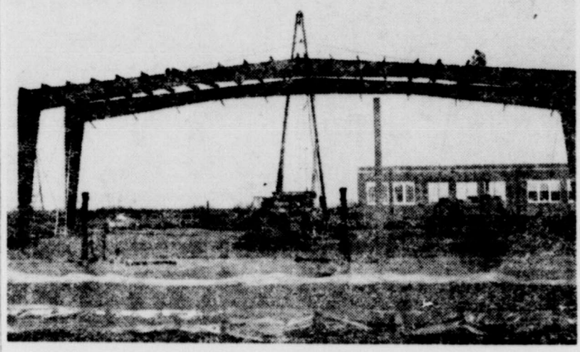
WORK PROGRESSING ON NEW GYM —Construction work is moving along for the Crowell Schools' new gymnasium. These pictures were made early last week showing the erection of the steel work on the building. In the top photo, Fred Glover and Joe Ray Setliff are shown atop the steel girders as Ennis Setliff and Edwin Edgin, on the ground, send up another piece of steel to be bolted on top of the girders. The bottom photo is an end view of the steel frame over the gymnasium portion of the building. Setliff Machine Shop of Crowell is erecting the steel framework for the general contractor.
