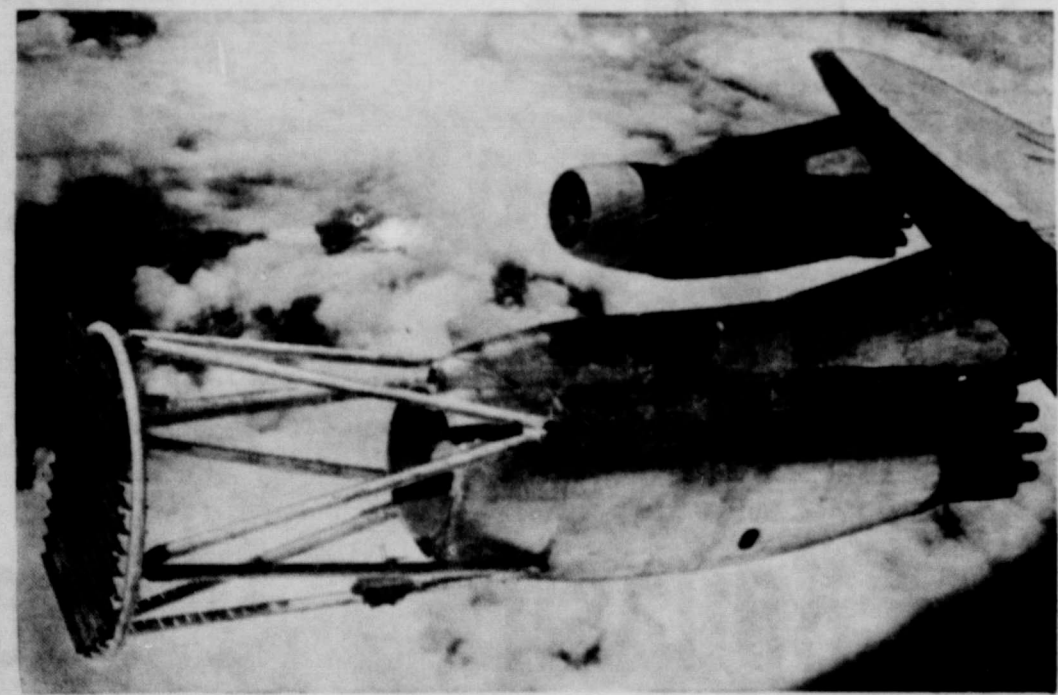
"AIR-CONDITIONING" THE ATMOSPHERE—A lowered mask installed in front of the No. 3 engine of a Boeing 707 prototype jet airliner "air-conditions" the atmosphere in front of the engine for tests in Seattle, Wash. Since natural icing conditions are hard to find, the 14 parallel bars are equipped with 109 spray nozzles which shoot water at the engine. After a quarter-inch of ice forms, the engine's hot-air de-icing system is tested.
