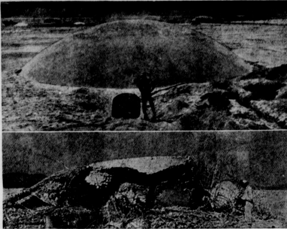
DOMES SHELTERS, a new design whose low cost and easy construction would adapt it to mass production, were tested at the Operation Plumbbob atomic tests in Nevada at pressures so great that 18 times those which a house is normally built to withstand. The 50-foot-diameter shelters may be seen before the blast in the upper photo. The lower photo shows one of the domes which was deliberately tested at a pressure so great that it would fall, so its weaker points could be studied. (NTO Lookout Mountain Lab Photo)
