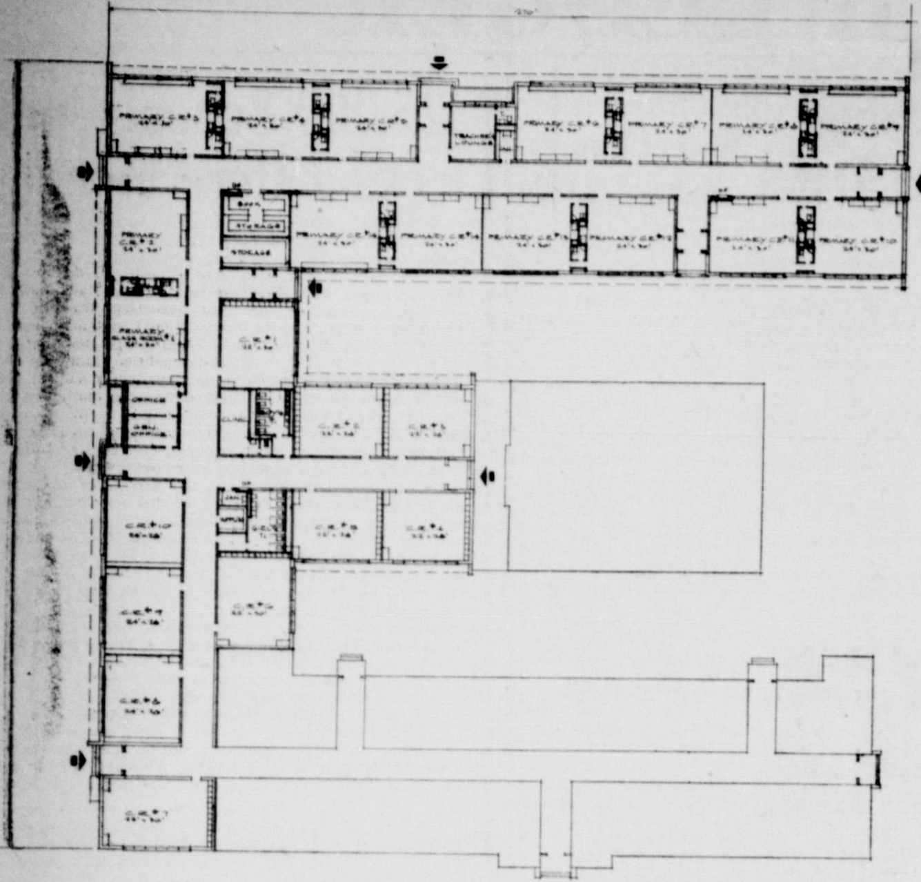
FLOOR PLAN
