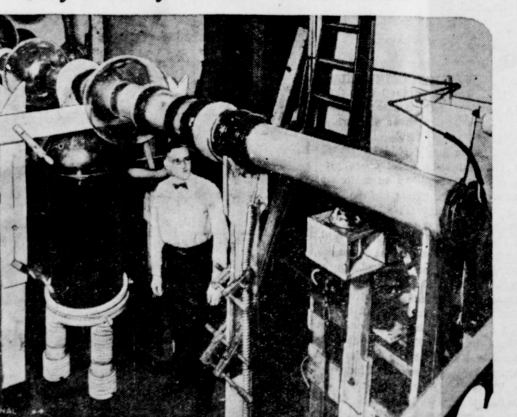
This giant 900,000-volt X-ray tube is being constructed in Schenectady, N. Y., under the direction of Dr. W. D. Coolidge for installation in the New York Memorial hospital where it will be used to combat cancer. The tube, which will be by far the largest ever built for medical use, is here photographed for the first time.
