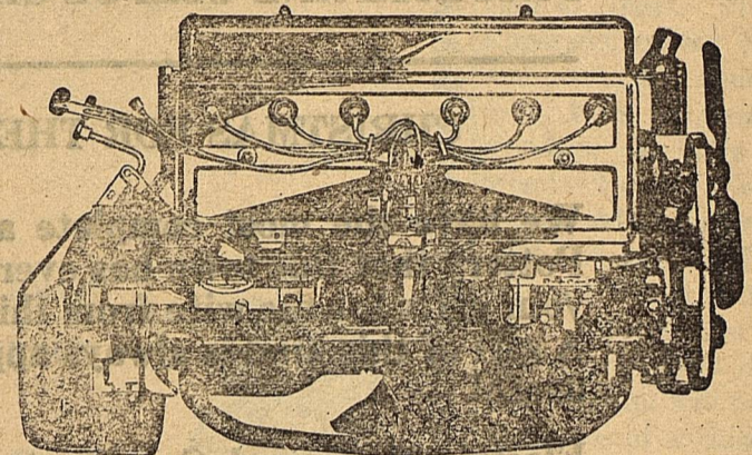
Chevrolet's new six-cylinder, fully enclosed valve-in-head engine has a high compression non-detonating head. Its piston displacement is 134 cu. in. and it develops 46 H. P. at low engine speed.
